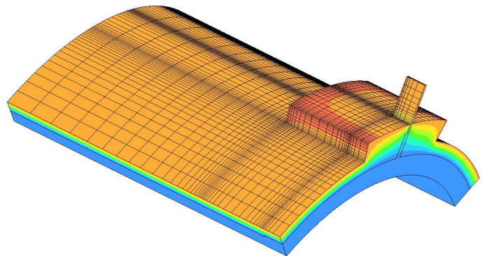
Temperature development of the structural element
